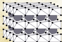
A Chelator Molecule
